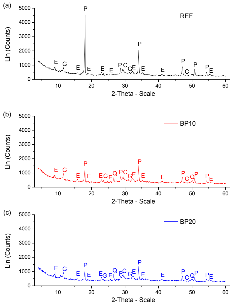
Fig. 9. (a) XRD spectrum for REF mortars; (b) XRD spectrum for BP10 mortars; (c) XRD spectrum for BP20 mortars. The meaning of the letters in the figure is the following: P Portlandite, C Calcite, E Ettringite, G Gypsum, Q Quartz.
