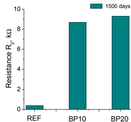
Fig. 7. Resistance R_2 results noted for REF, BP10 and BP20 mortars.
