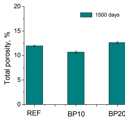
Fig. 2. Results of total porosity noted for the studied mortars. Error bars in this figure and in the following represents the standard deviation.
