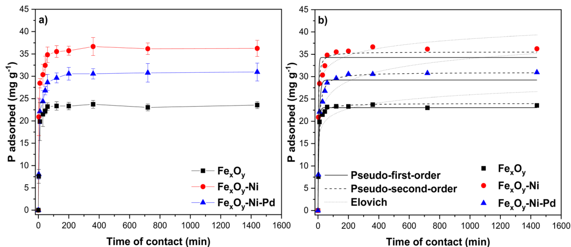
Fig. 8 Kinetics of P adsorption on Fe x O y , Fe x O y -Ni, and Fe x O y -Ni-Pd nanoparticles (a), and model fitting lines of the experimental data (b). Initial P concentration 200 mg L -1 in 10 mmol L -1 NaCl; initial pH 5.5 ± 0.2; reaction volume 20 mL. Error bars denote standard deviation; n = 3 .
