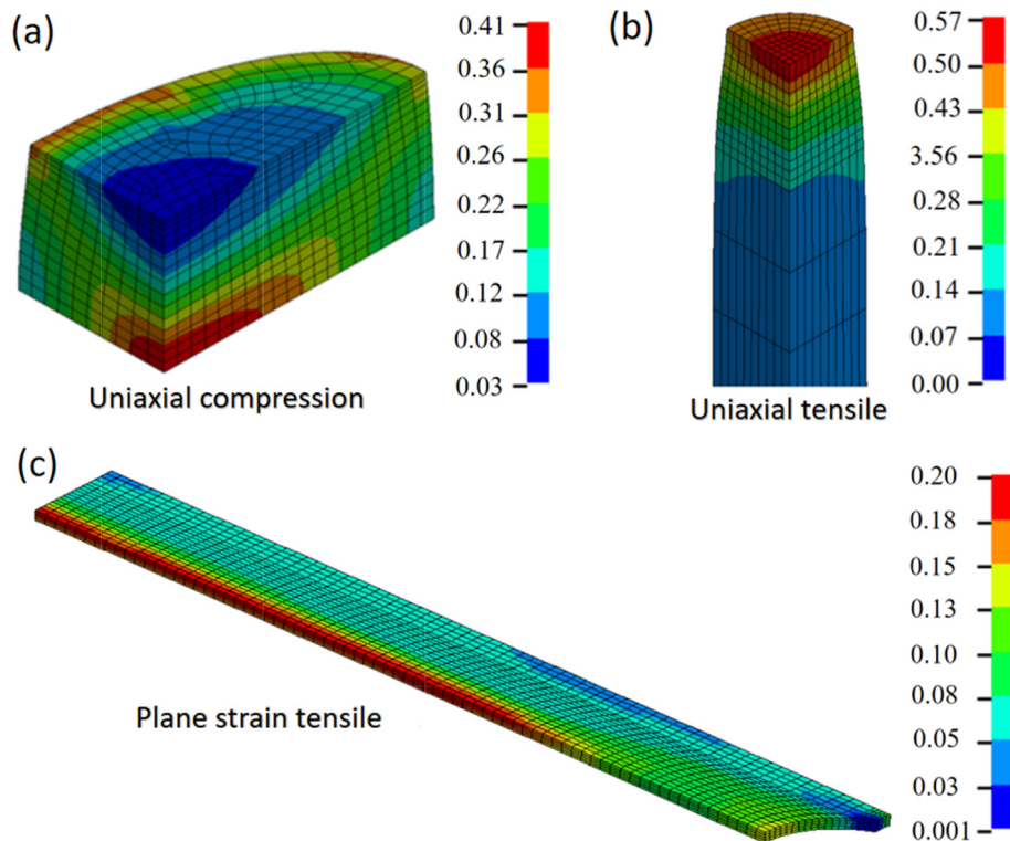
Fig. 5 – Contour plot for the equivalent strain of the investigated samples, noting maximum values reached are: 95% of the maximum axial fracture deformation for (a) compressive sample and at the onset of fracture for tensile loadings: (b) uniaxial, and (c) plane strain.
