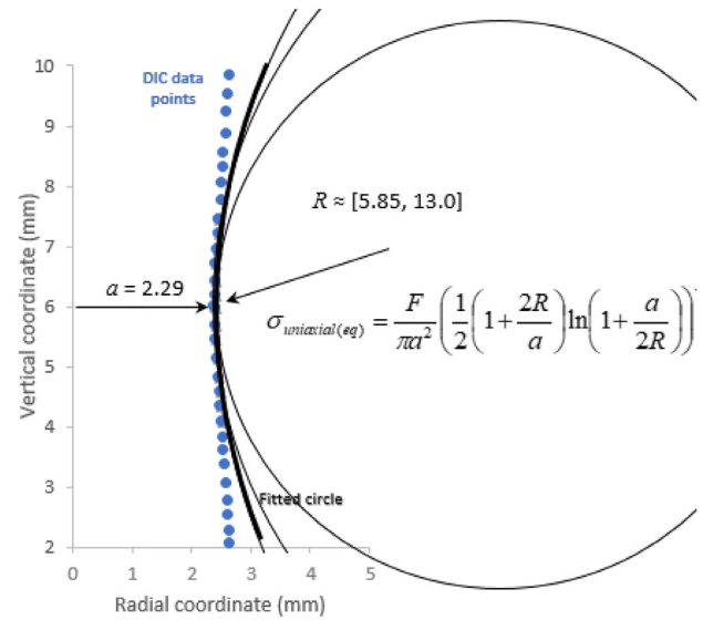
Fig. 6 – Experimental neck of the tensile cylinder at maximum elongation showing difficulties in accurately measuring the radius ( R ) required to apply the Goodman corrector.
