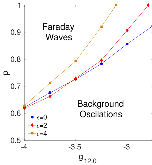
Fig. 7. Influence of the modulation amplitude p on the Faraday wave stability. Phase diagram in the plane \{g_{12,0}, p\} where the Faraday wave are elicited. Three values of \epsilon are considered: (0, 2, 4). The rest of the parameters are fixed as in Fig. 1.
