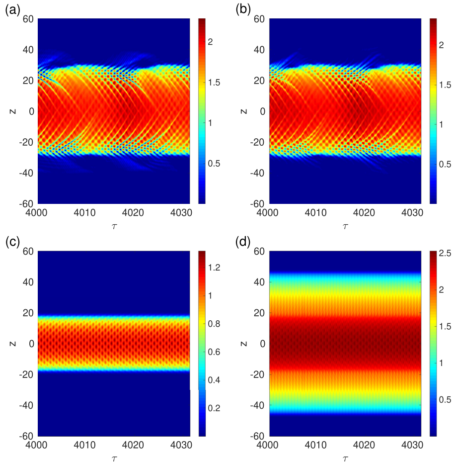
Fig. 6. Space-time evolution of the individual densities n_1 (left panels) and n_2 (right panels). The upper row corresponds to \epsilon = 1.0 and a synchronized state ( C_P \approx 1 ). The lower row corresponds to \epsilon = 6.0 , the two fields are not synchronized ( C_P \approx 0.7 ). Here we have set g_{12,0} = -3.4 and the rest of the parameters are fixed as in Fig. 5.
