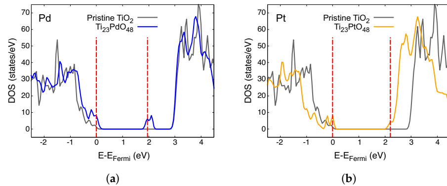
Figure 5. Density of states of paramagnetic Ti 23 AO 48 : (a) A = Pd; (b) A = Pt. The DOS for pristine TiO 2 is plotted in gray in each case. The vertical red dashed lines are visual guides with which to identify the band gap.
