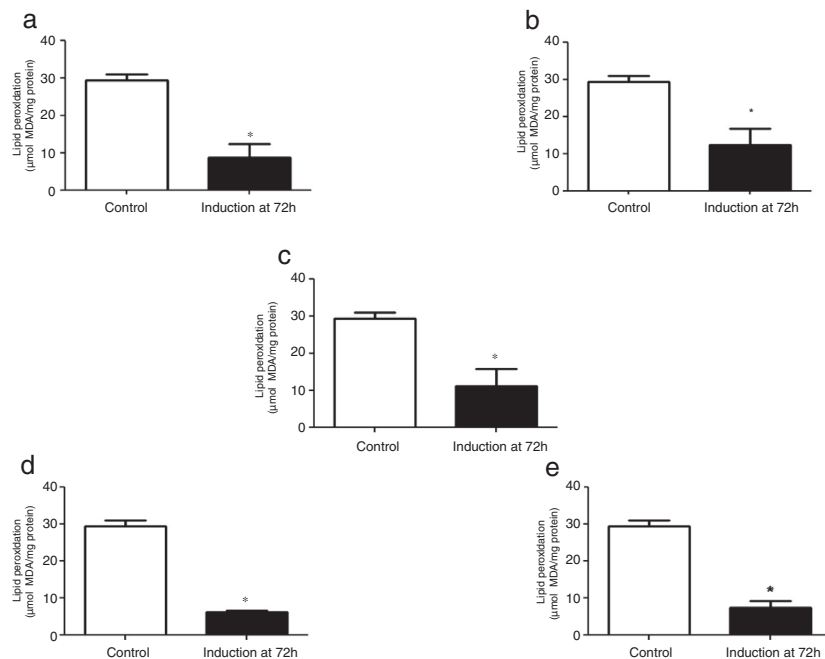
Fig. 2 – Effects of different culture conditions on the lipid peroxidation level. (a) 14 °C – 1%M, (b) 14 °C – 2%M, (c) 18 °C – 1.5%M, (d) 22 °C – 1%M, (e) 22 °C – 2%M. Each bar represents the mean \pm SD ( n = 3 ). Statistical analysis by paired t-test. * p < 0.05 (0 h vs. 72 h).
