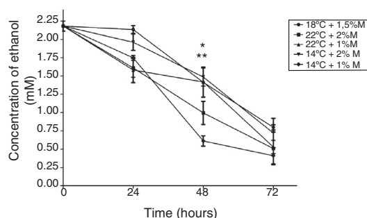
Fig. 5 – Ethanol concentration. Representative graphic of the ethanol concentration in different culture conditions. Each point represents the mean \pm SD ( n = 3 ). Statistical analysis by two-way ANOVA–Bonferroni's post-test. * p < 0.05 (22 °C + 2%M vs. all other conditions); ** p < 0.05 (14 °C + 1%M vs. all other conditions).
