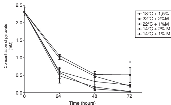
Fig. 4 – Pyruvate concentration. Representative graphic of the pyruvate concentration in different culture conditions. Each point represents the mean \pm SD ( n = 3 ). Statistical analysis by two-way ANOVA-Bonferroni's post-test. * p < 0.05 (14 °C + 1%M vs. all other conditions); ** p < 0.01 (18 °C + 1.5%M vs. 22 °C + 1%M, 14 °C + 2%M, 14 °C + 1%M); *** p < 0.01 (22 °C + 2%M vs. 22 °C + 1%M, 14 °C + 2%M, 14 °C + 1%M).
