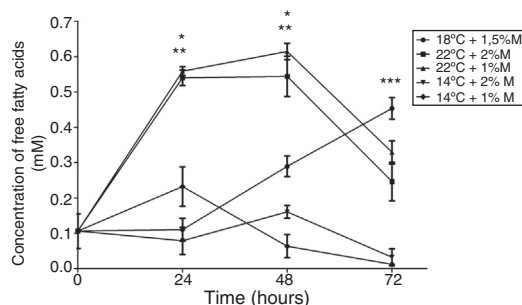
Fig. 7 – Free fatty acid concentration. Representative graphic of the free fatty acid concentration in different culture conditions. Each point represents the mean \pm SD ( n = 3 ). Statistical analysis by two-way ANOVA–Bonferroni's post-test. * p < 0.001 (22 °C + 2%M vs. 18 °C + 1.5%M, 14 °C + 2%M, 14 °C + 1%M); ** p < 0.001 (22 °C + 1%M vs. 18 °C + 1.5%M, 14 °C + 2%M, 14 °C + 1%M); *** p < 0.05 (18 °C + 1.5%M vs. all other conditions).
