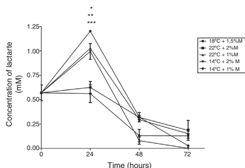
Fig. 6 – Lactate concentration. Representative graphic of the lactate concentration in different culture conditions. Each point represents the mean \pm SD ( n = 3 ). Statistical analysis by two way ANOVA–Bonferroni's post-test. * p < 0.05 (14 °C + 1%M vs. all other conditions); ** p < 0.01 (18 °C + 1.5%M vs. 22 °C + 1%M, 14 °C + 2%M, 14 °C + 1%M); *** p < 0.01 (22 °C + 2%M vs. 22 °C + 1%M, 14 °C + 2%M, 14 °C + 1%M).
