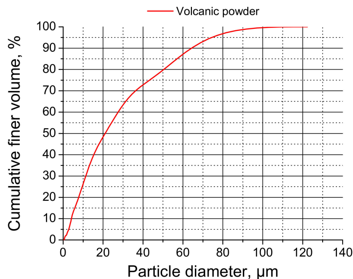
Figure 1. Size distribution of particles of studied powder.
