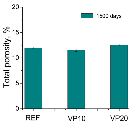
Figure 3. Total porosity results for the analyzed series.
