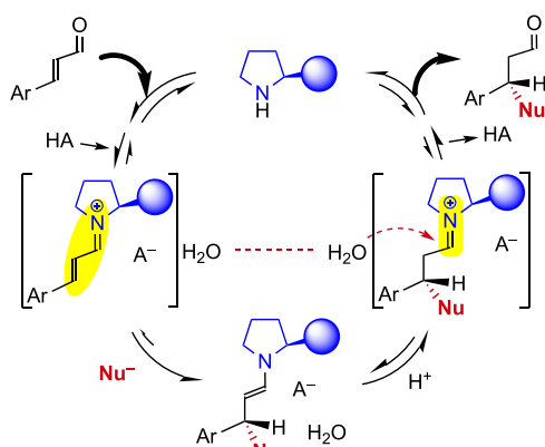
Scheme 1. Organocatalytic Reaction of Enals, through Eniminium Ions, with Nucleophiles
