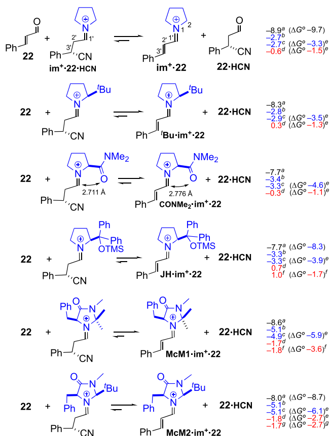
Scheme 8. Exchanges of Known Secondary Amines between 22 and Iminium Ions from Adducts a–g
