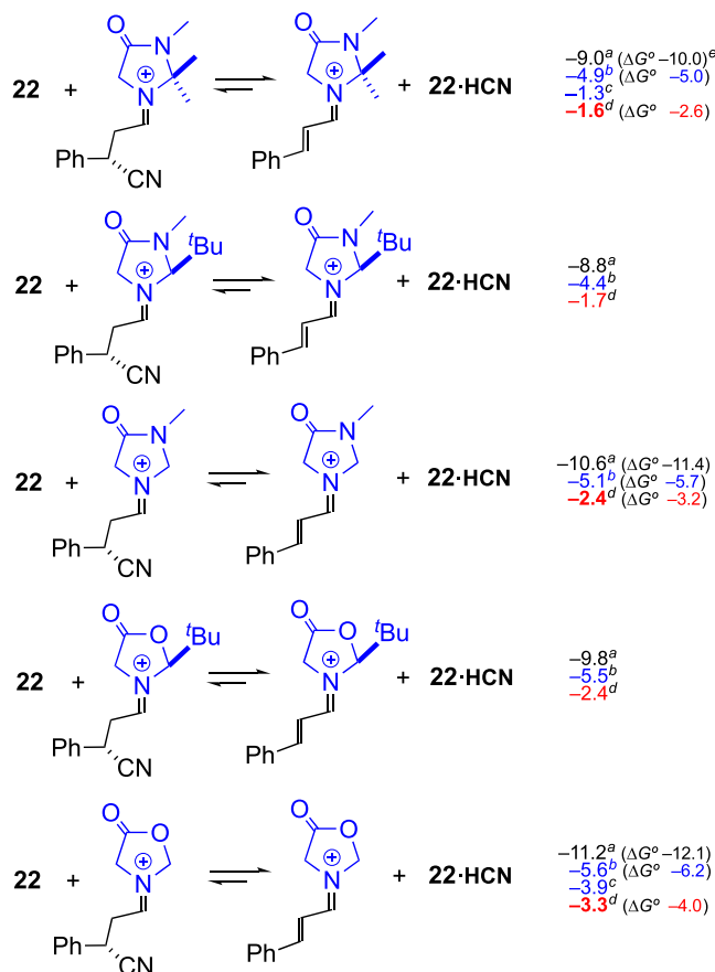
Scheme 9. Exchanges of Imidazolidinones and Oxazolidinones between 22 and Iminium Ions from Adducts a–e
