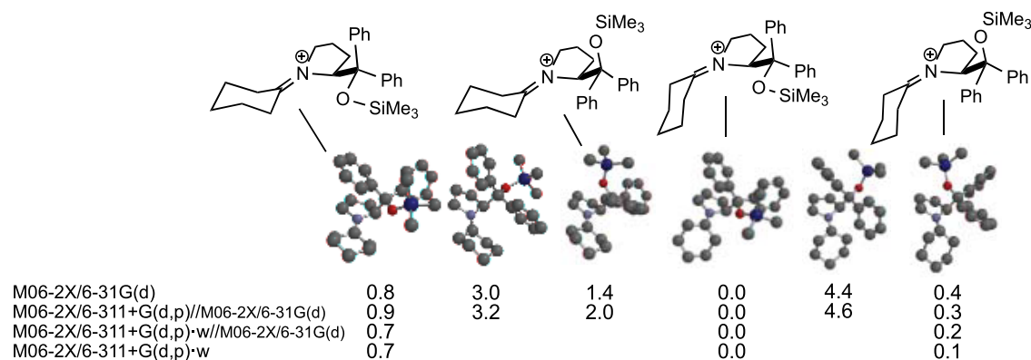
Scheme 6. Main Conformers of JH·im + ·1, the Iminium Ion from the JH Catalyst and 1 a
