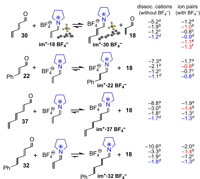
Scheme 4. Exchange of Pyrrolidine between Enals, Dienals, and Trienals, and either Their Iminium Ions or Their Tetrafluoroborates a–f
