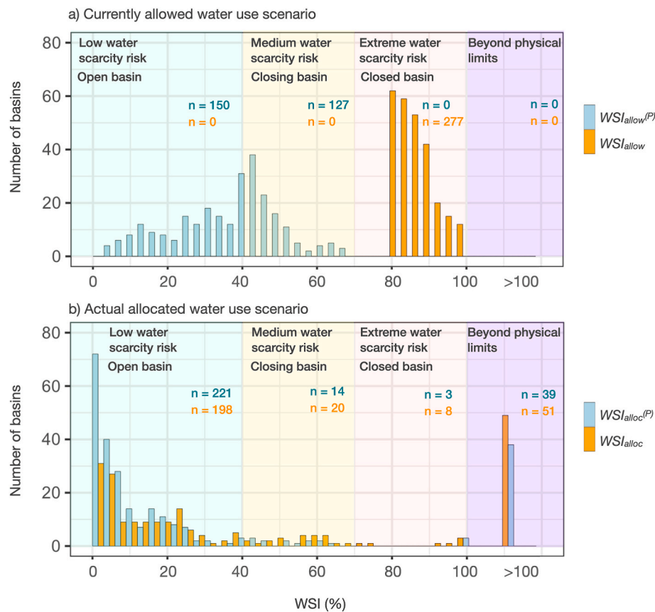
Fig. 5. WSI computed based on permanent and total withdrawals, under current allowed (panel a) and allocated water-use scenarios (panel b). The WSI values are classified following Table 1. The numbers of basins within in each WSI category are presented in blue and orange for permanent and total withdrawals, respectively. (For interpretation of the references to colour in this figure legend, the reader is referred to the Web version of this article.)
