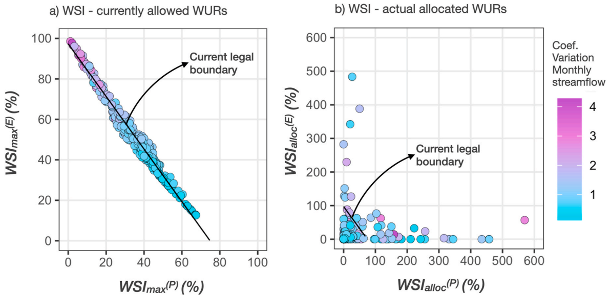
Fig. 4. WSI computed from permanent and eventual WURs, under currently allowed (panel a) and actual allocated scenarios (panel b).
