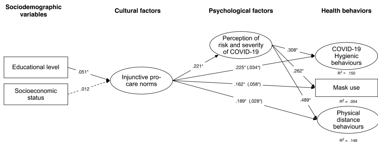
Figure 1. Model (invariant for the Chilean, Mexican, and Colombian sample) predicting self-care COVID-19 behaviors.
