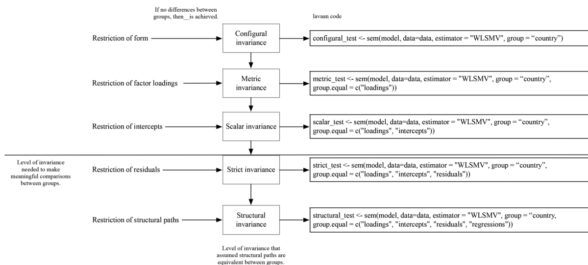
Figure 2. Overview of the statistical analysis to assess invariance between countries with their respective Llavaan code.
