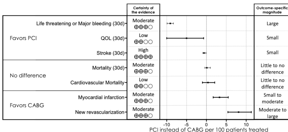
Fig. 2. Summary of absolute risk differences between PCI and CABG from meta-analysis.
