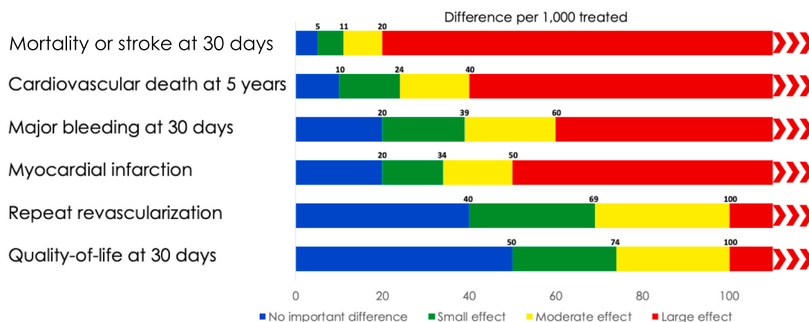
Fig. 1. Outcome thresholds.
