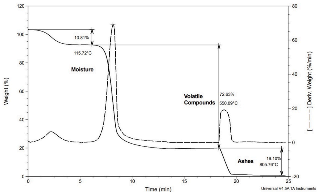
Fig. 4. Results of the thermal stability test.
